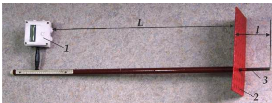
Fig. 3. Depth gauge: 1 – registration and information block; 2 - support; 3 - moving rod
