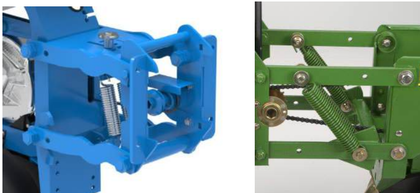
Fig. 2. Springs, with the help of which you can change the degree of pressure on the soil
